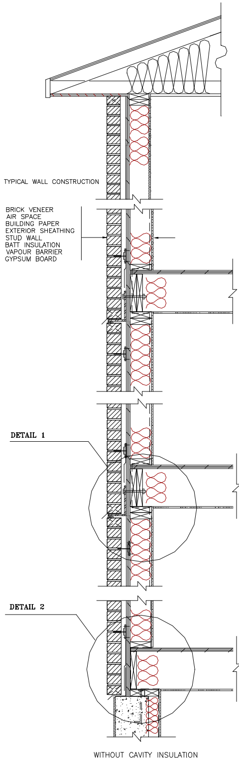
Detail 7.1 – Typical Wood Frame Construction Apartment Building
